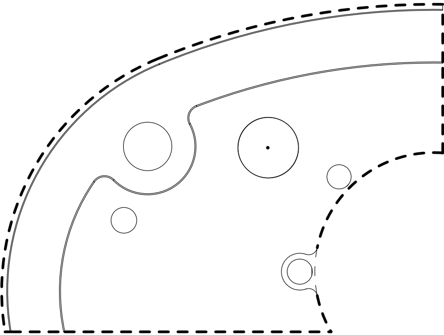
Drilling Template For Step 6.
